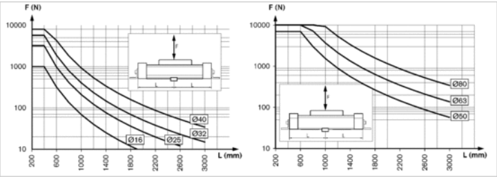
Max. support span L [mm] as a function of F [N] at a deflection of 0.5 mm
